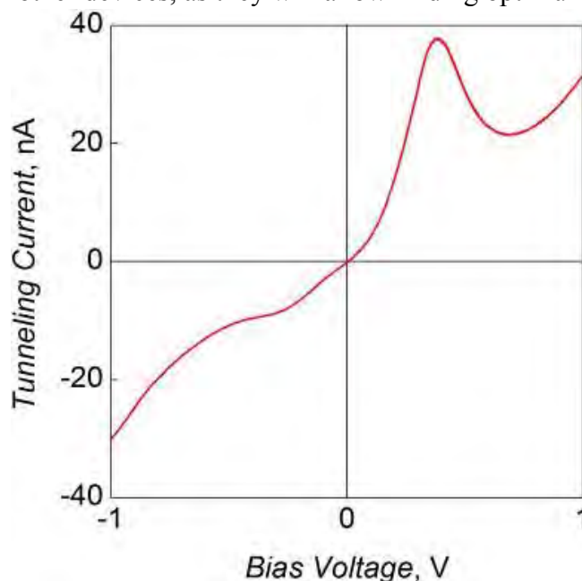
Fig. 29 I(V) characteristics of a SLG/4L\text{-BN}/SLG device. Adapted from Ref. [106].
