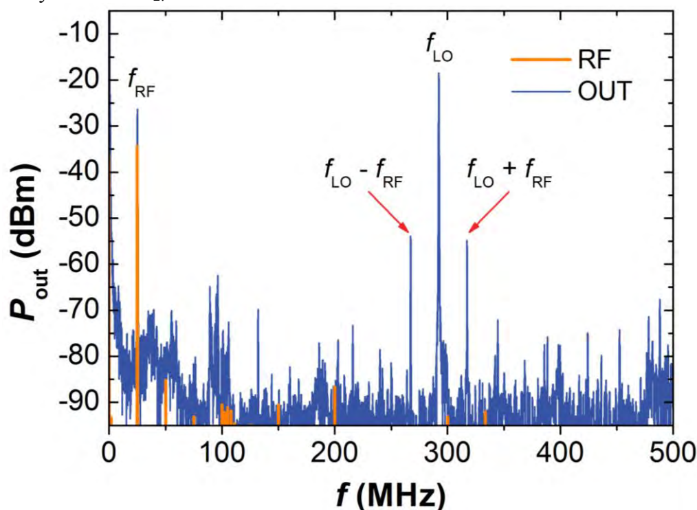
Fig. 65 Power spectrum of the output signal of a stand-alone graphene mixer at V_{DD} = 2.5\text{ V} . The signal frequencies are f_{LO} = 292\text{ MHz} and f_{RF} = 25\text{ MHz} . Apart from the signals discussed in the text, the output signal also contains a frequency component at f_{RF} , from the amplification of the RF signal by inverter 4 [1102].
