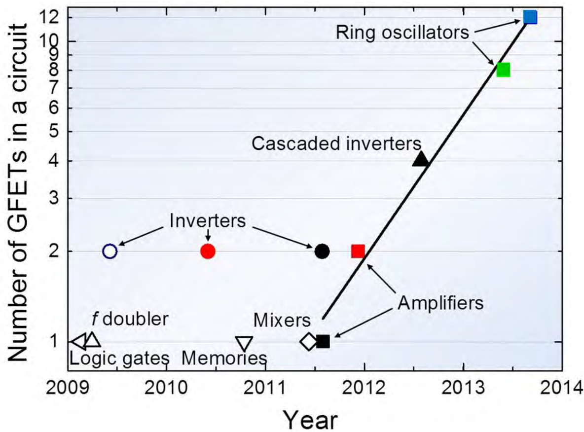
Fig. 58 Transistor count in graphene circuits with |A_v| < 1 (open symbols) and |A_v| > 1 (filled symbols). The linear fit is performed only on circuits with over-unity RT AC |A_v| . From this, a graphene Moore's law is obtained: the number of GFETs on a chip currently doubles approximately every 8 months. However, it is unlikely that this will hold in the near future. Values taken from: \triangleleft [1149], \triangle [1150], \nabla [1140], \diamond [11], \blacksquare [1142], \blacksquare [1143], \circ [1151], \bullet [1141], \bullet [1129], \blacktriangle [1144], \blacksquare [1155], \blacksquare [1102]. Adapted from Ref.1208.
