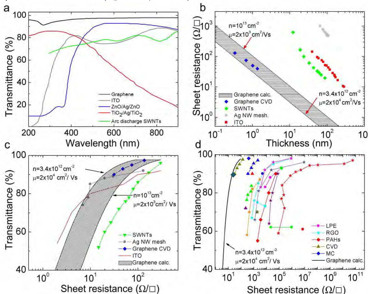
Fig. 92 a) Transmittance of graphene compared to different TCs: GTCFs 7 , SWNTs 1782 , ITO 1780 , ZnO/Ag/ZnO (ref. 1785) and TiO 2 /Ag/TiO 2 (ref. 1763). b) Thickness dependence of R_s for graphene compared to some common materials; The blue rhombuses show roll-to-roll GTCFs based on CVD-graphene 7 ; red squares, ITO 1780 ; grey dots, metal nanowires 1780 ; green rhombuses, SWNTs 1782 . Two limiting lines for GTCFs are also plotted using typical values for n and \mu reported in the graph. c) Tr vs R_s for different TCs compared to graphene; blue rhombuses, roll-to-roll GTCFs based on CVD-graphene 7 ; red line, ITO 1780 ; grey dots, metal nanowires 1780 ; green triangles, SWNTs 1782 . Shaded area enclosed by limiting lines for GTCFs calculated using n and \mu as in b. d) Tr vs R_s for GTCFs grouped according to production strategies: LPE, RGO, organic synthesis using PAHs, CVD, and MC. triangles, CVD 7,9,824 ; the dark cyan rhombus is a hybrid metallic grid/graphene film 1786 ; blue rhombuses, micromechanical cleavage (MC) 623 ; red rhombuses, organic synthesis from polyaromatic hydrocarbons (PAHs) 710 ; dots, liquid-phase exfoliation (LPE) of pristine graphene 35,623,624,642 ; and stars, reduced graphene oxide (RGO) 679,688,706,1788,1797 . A theoretical line is also plotted for comparison. Adapted from Ref. [995].
