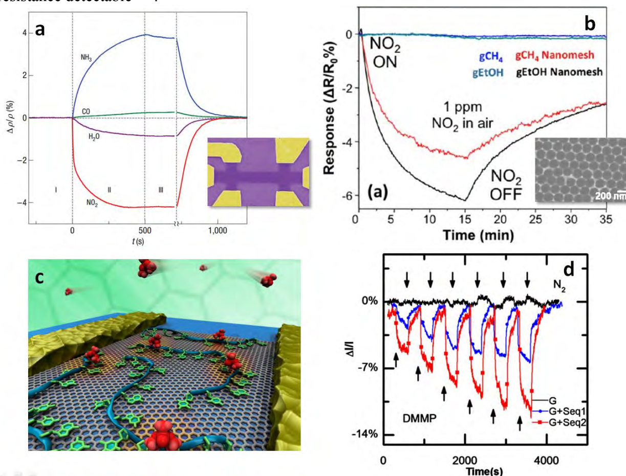
Fig. 87 (a) Ref. 1648 demonstrated sensitive chemoresistive response using graphene field effect devices (inset), with a dependence on the type of analyte. (b) Nanopatterning can enhance the sensitivity of graphene chemical sensors. Ref. 1706 showed that large-area nanopatterning (inset) using colloidal lithography, could lead to a strongly increased response to various gas molecules. The \text{gCH}_4 and \text{gEtOH} labels refer to graphene grown with methane and ethanol, respectively. The higher response of \text{gEtOH} samples was related to a higher defect density 1648 . (c) Decoration with DNA molecules of a graphene field effect device can affect the chemoresistive response according to the specific DNA sequence. (d) Normalized changes in current vs time for ssDNA-graphene vapor responses. Lower arrows indicate introduction of analyte at progressively larger concentrations, while upper arrows indicate flushing with pure carrier gas. Graphene devices (black data) show very weak
