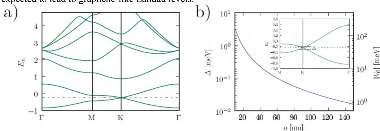
Fig. 19 a) AG Minibands (energy is in meV) with a lattice period a = 60\text{ nm} , r_0 = 0.2a ( r_0 is the width of the potential well) and V_0 = 5\text{ meV} . A dash-dotted line is drawn at the Dirac-point energy. b) Energy width ( \Delta ) of the linear part of the spectrum near the Dirac point as a function of a . V_0 is varied correspondingly (see the right vertical axis) in order to obtain an isolated Dirac point, i.e. without any other state inside the bulk Brillouin zone at the Dirac-point energy. Inset: magnification of the energy bands in panel a) around the Dirac point energy. The blue dashed lines mark the energy limits of the linear dispersion approximation. Adapted from Ref. [260].
