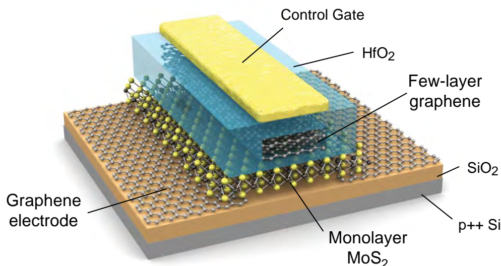
Fig. 66 MoS_2 /graphene heterostructure memory layout. (a) 3d schematic view of the memory device based on 1L- MoS_2 semiconducting channel, SLG contacts and FLG floating gate. The FLG floating gate is separated from the channel by a thin tunnelling oxide and from the control gate by a thicker blocking oxide.
