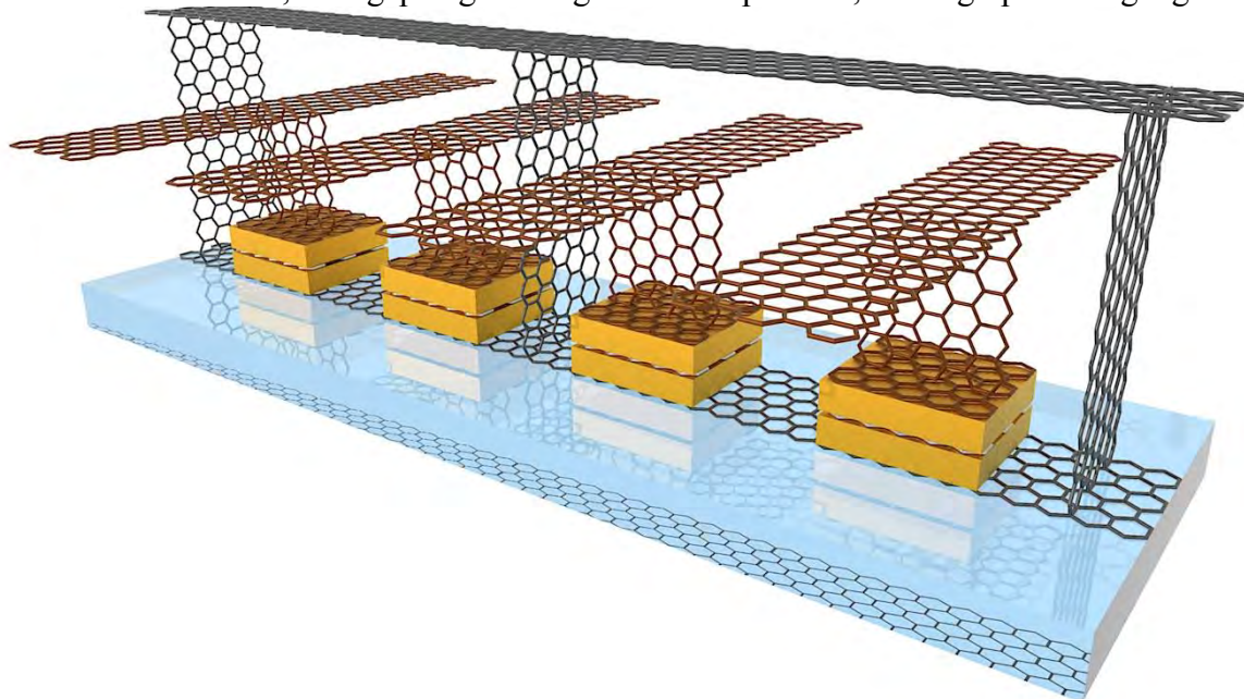
Fig. 60 Two cells graphene NOR gate flash memory. Graphene is used for conductive FET
