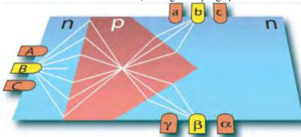
Fig. 89 Prism-shaped focusing beam-splitter in a ballistic graphene n-p-n junction. Electrons emitted from contact B are distributed between contacts b and \beta . Adapted from Ref. [143].
