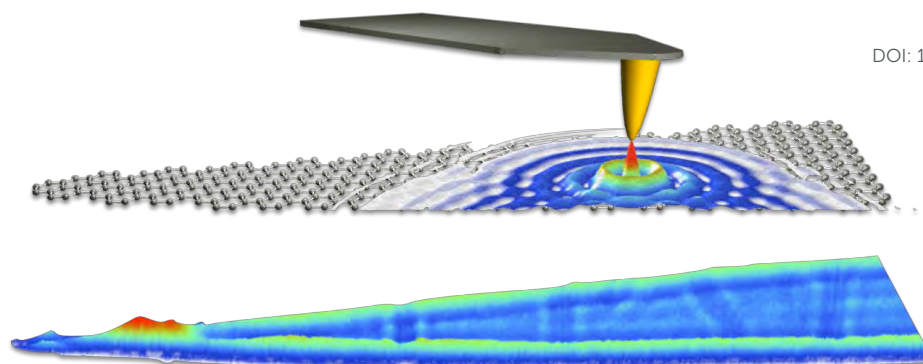
Fig. 83 Top: Schematic of configuration used to launch and detect propagating surface waves. Bottom: Near-field amplitude image acquired for a tapered GNR on top of 6H-SiC. The imaging wavelength is 9.7\mu\text{m} . The tapered ribbon is 12\mu\text{m} long and up to 1\mu\text{m} wide [adapted from Ref. 1326].
